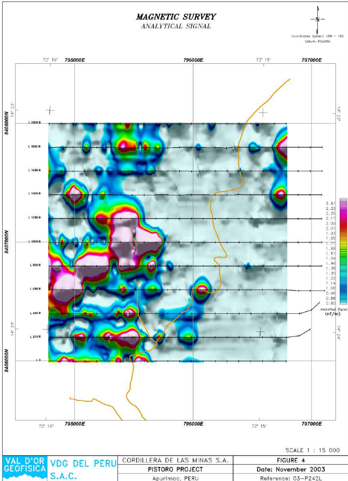
Figure 49: Pistoro Norte Total Magnetic Field Analytical Signature Map
