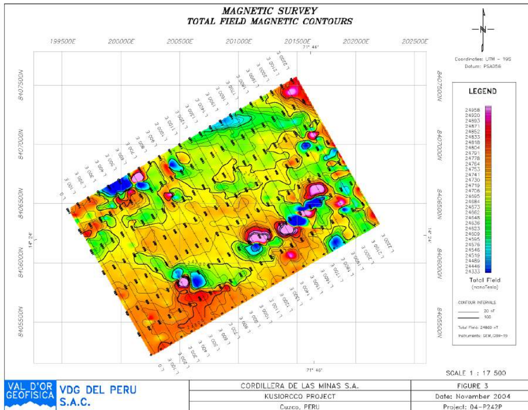
Figure 40: Kusiorecco Total Magnetic Field Map
