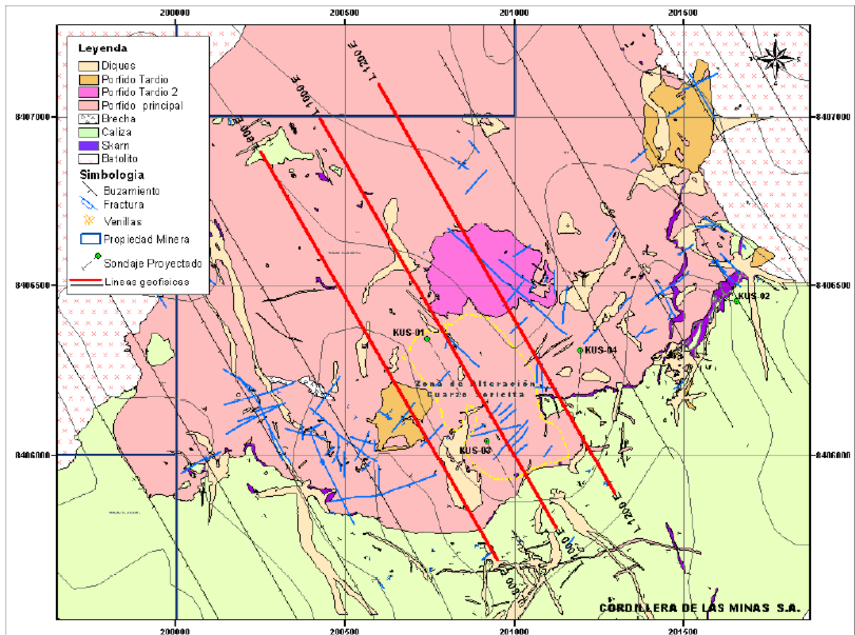
Figure 39: Kusiocco Geology
