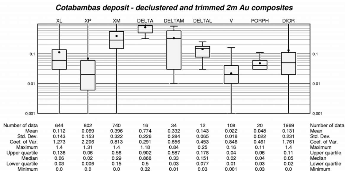
Figure 19: Au statistics of 2m composite grades
