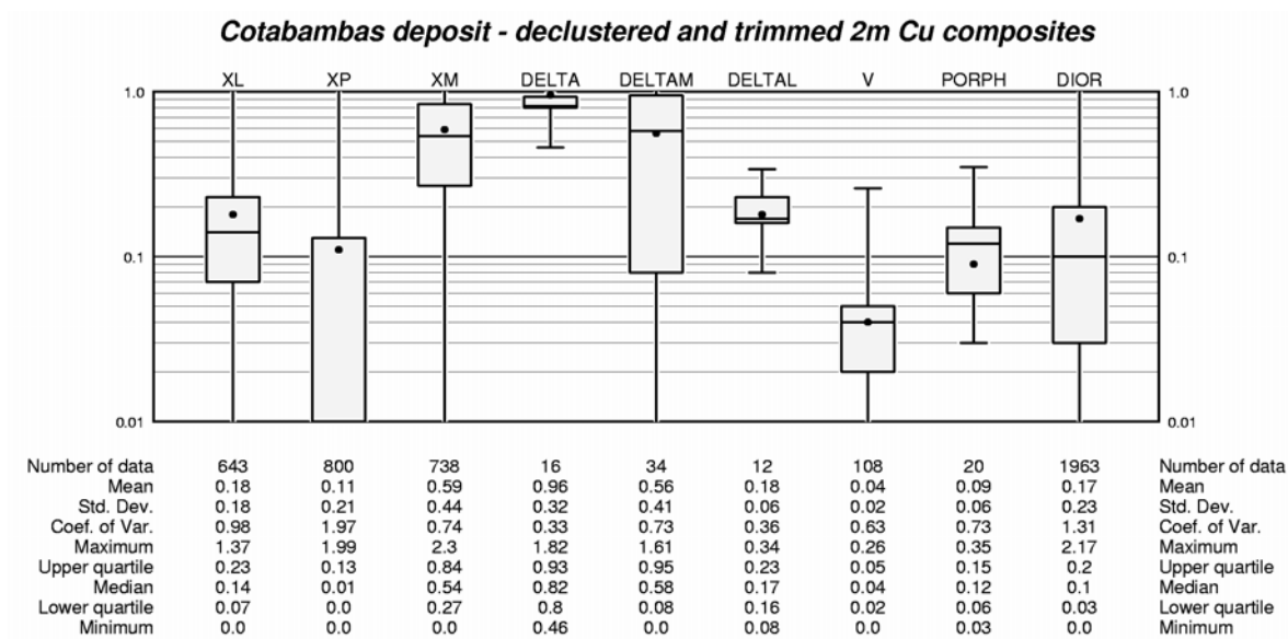
Figure 18: Cu statistics of 2m composite grades
