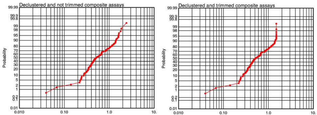
Figure 31: Log-probability plots of Cu composite grades
