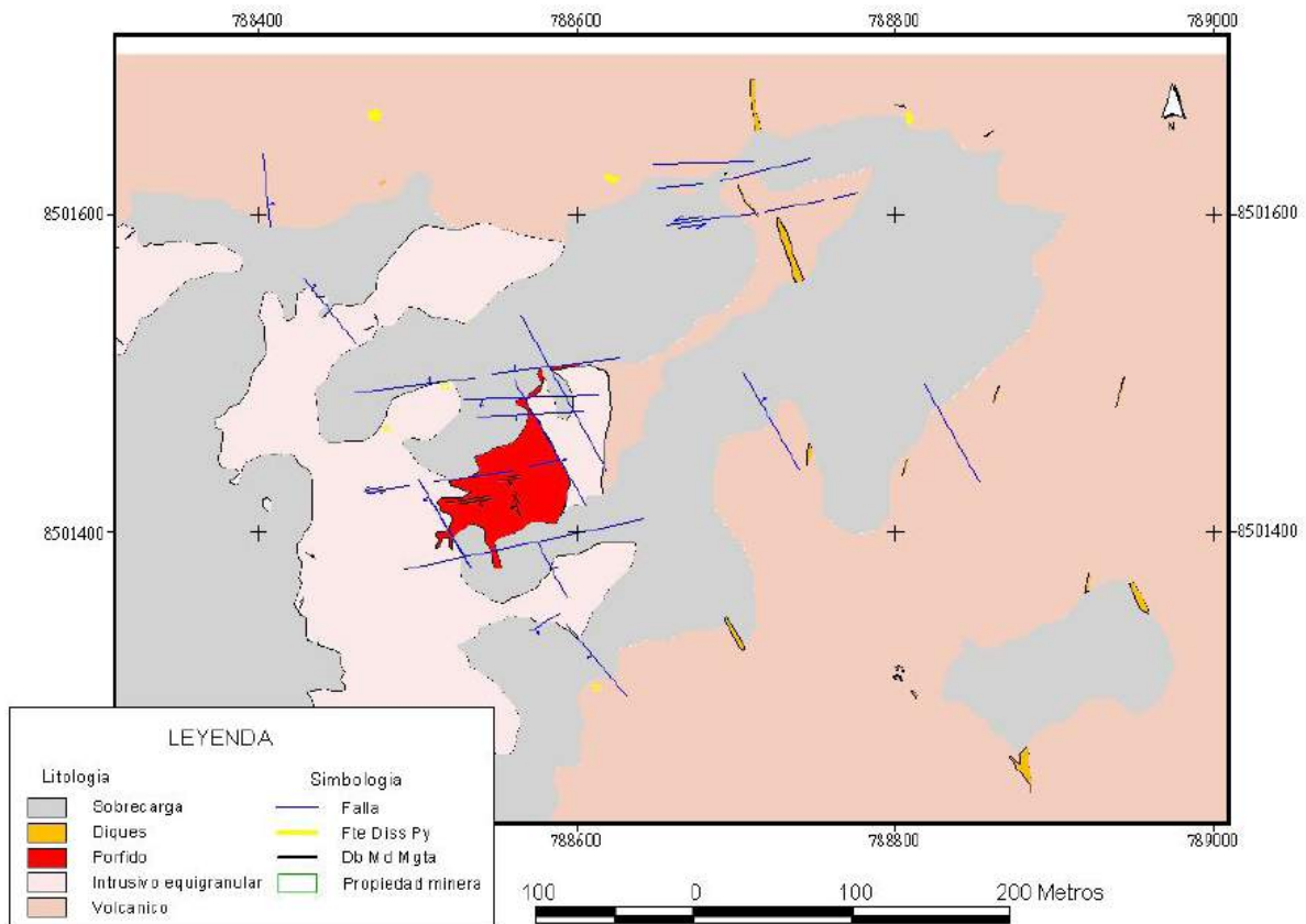
Figure 58: Geology of Morosayhuas area of porphyry outcrop
