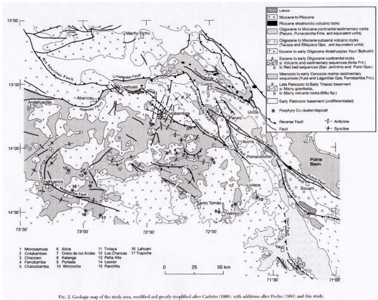
FIG. 2. Geologic map of the study area, modified and greatly simplified after Carlotto (1998), with additions after Pecho (1981) and this study.
