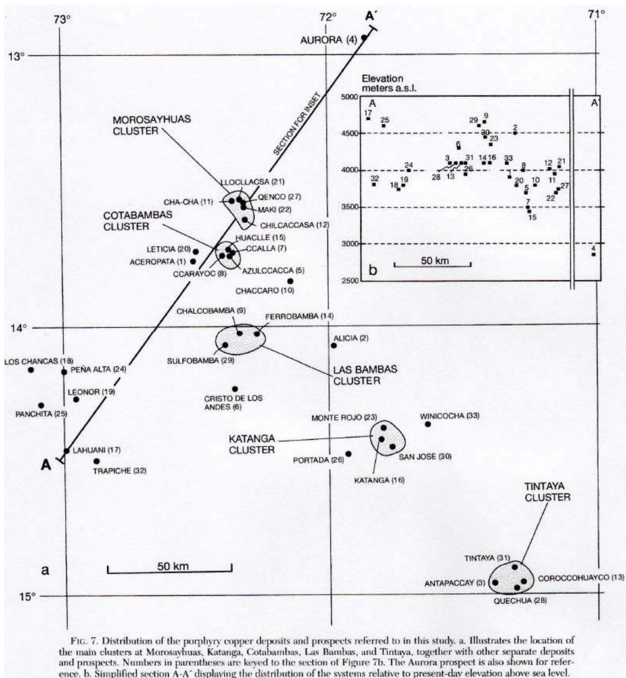
Figure 4: Distribution of porphyry copper deposits (J.Perello,V.Carlotto et al., 2003)
