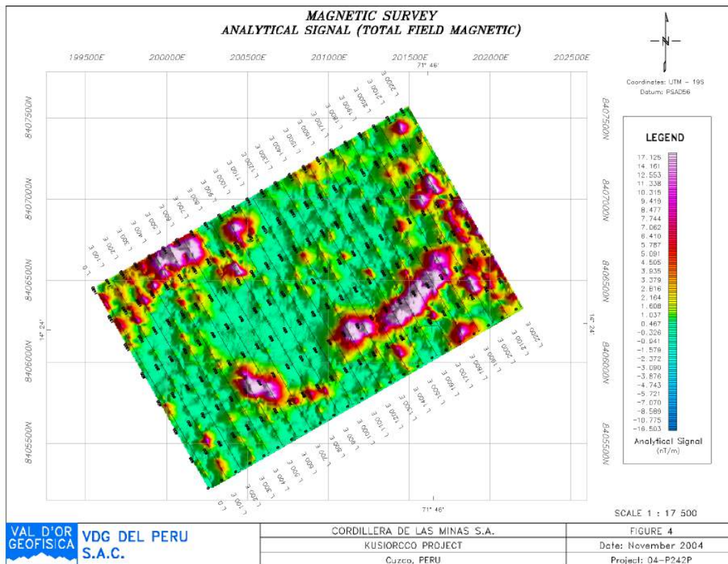
Figure 41: Kusiorecco Total Magnetic Field Analytical Signature Map
