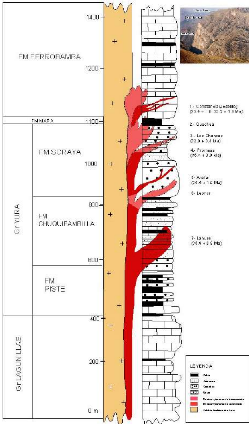
Figure 26: Stratigraphic section of the Antilla deposit setting (from CDLM 2004 Annual report)
