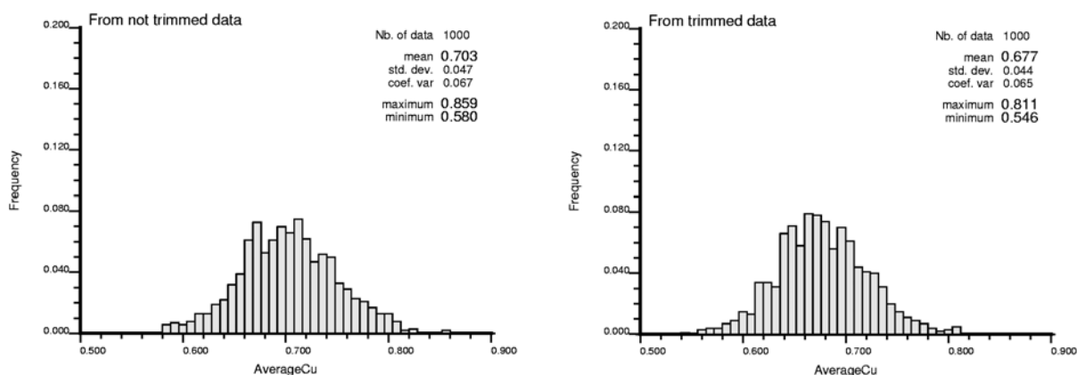
Figure 32: Distribution of global average grades
