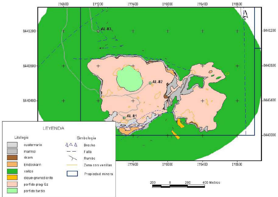
Figure 35: Geology and drill hole Locations Alicia Prospect
